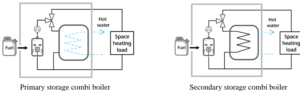
Figure B1 Primary and secondary storage combi boilers
