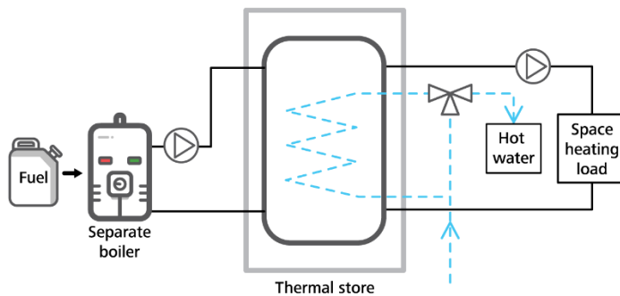
Figure B3 Integrated thermal store
